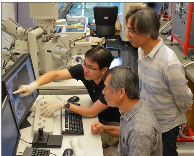
Figure D-13 Clay analysis using scanning electron microscopy (from right to left order: Master Kyoshi Matsuda, Master Yoneshi Matsuda, Dr. Kenichi Sajiki)
