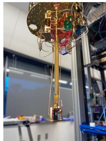
Figure 1. A test device installed in a dilution refrigerator that cools the device down to approximately 10 millikelvin temperature.
