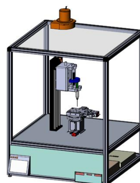
Figure 2. 3D-CAD design of hybrid fabrication technology
