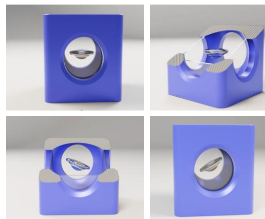
Figure 2: Schematic of the magnetically tunable lens in different configurations, with changing focal length, pitch and yaw. The shape corrects for spherical aberration.
